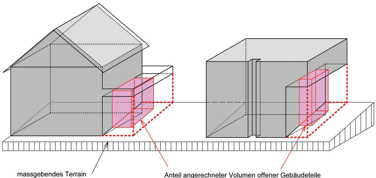
Figur 8.3 Baumassenziffer
